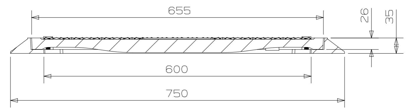
SECTION C - C
